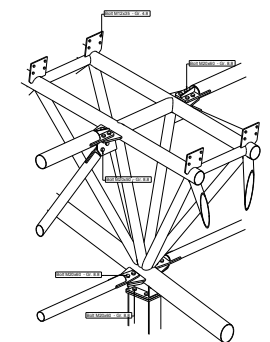
3D VIEW - 02 SCALE 1/10
