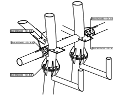
3D VIEW - 01 SCALE 1/10
