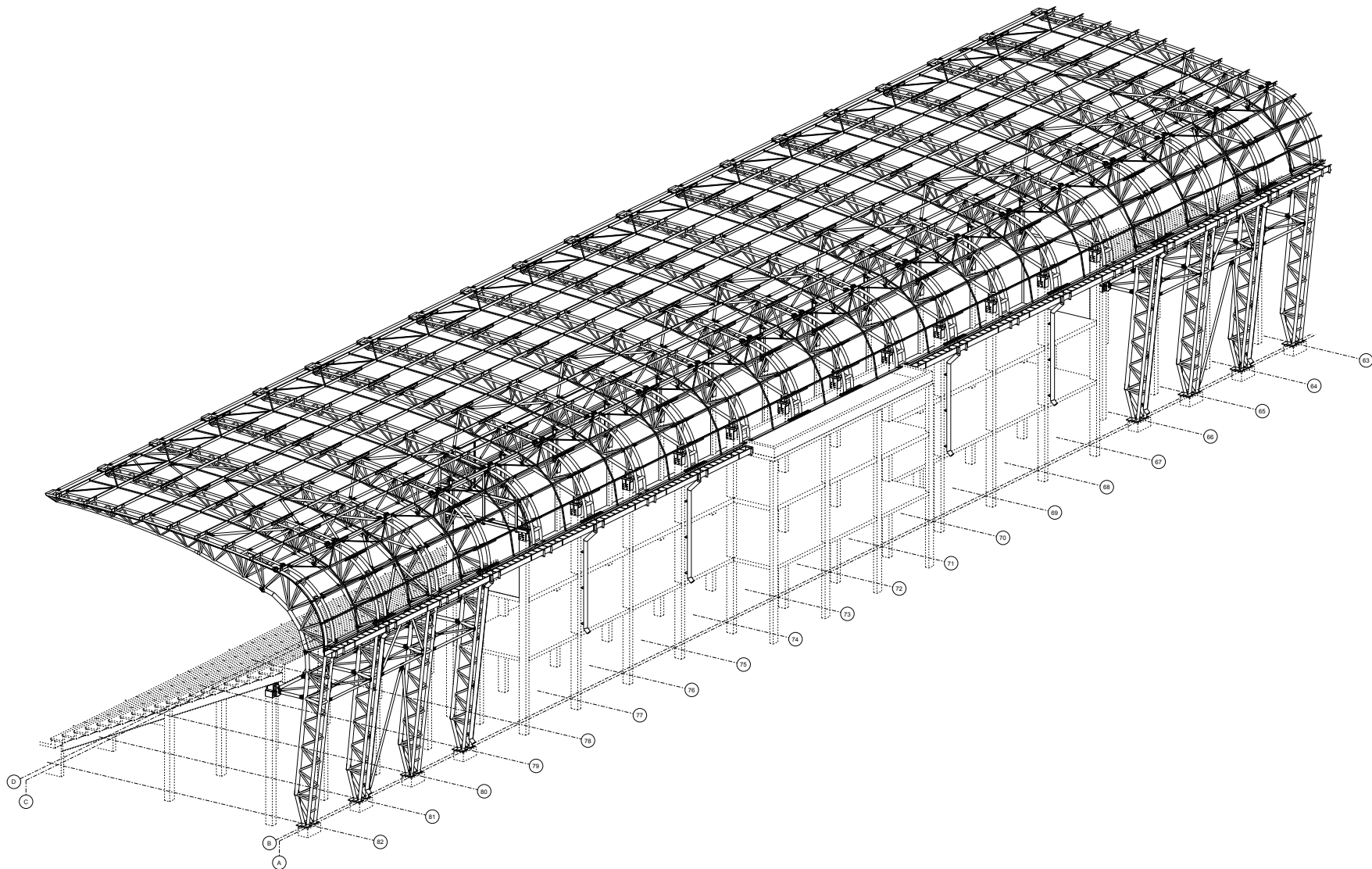
WEST PAVILION - ISOMETRIC VIEW. SCALE 1/5
