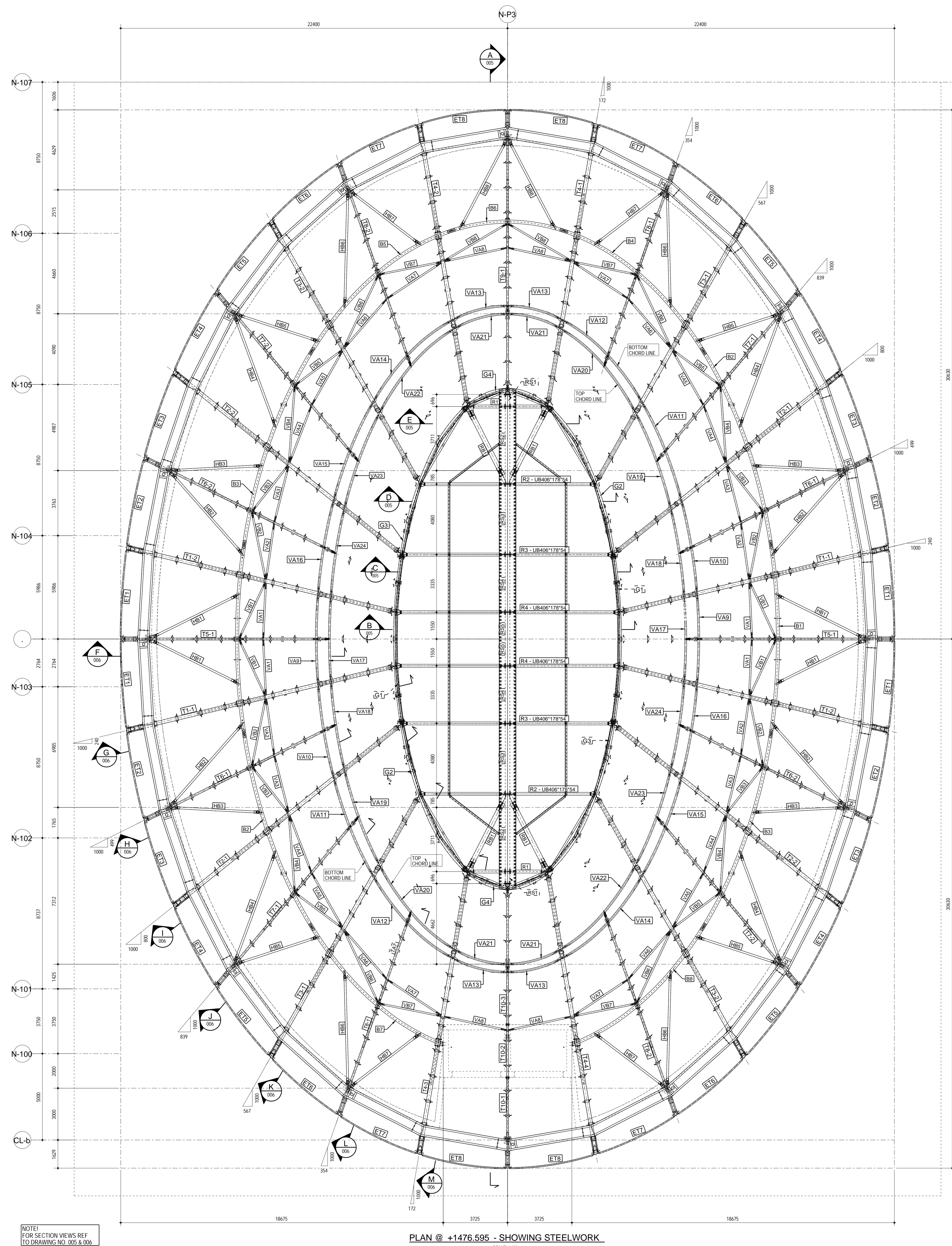
PLAN @ +1476.595 - SHOWING STEELWORK SCALE 1:100
